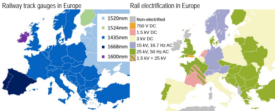
Figure 3.2 Different types of railway track gauges and electrification systems in Europe
